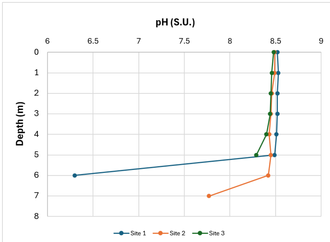
Figure 1. Graph of pH measurements (reported in standard units) collected with depth on July 22, 2026. Pumphouse measurement only reported in Table 1.
