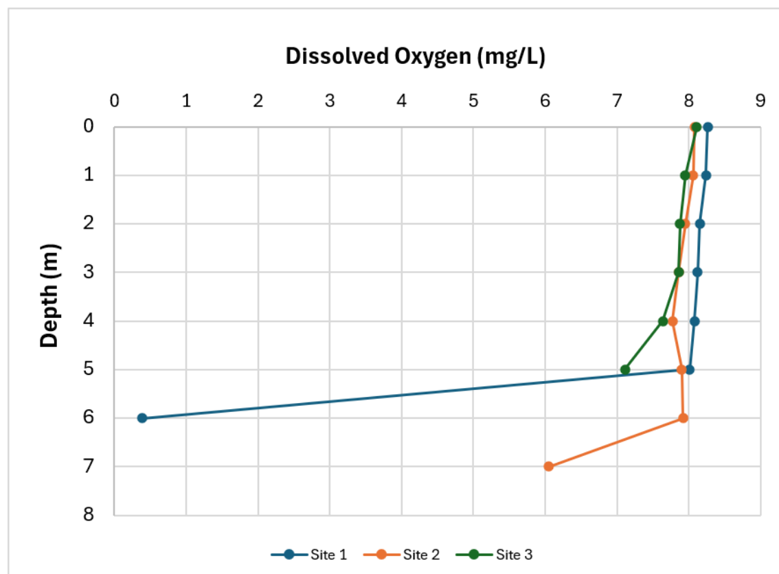
Figure 3. Graph of dissolved oxygen measurements (reported in mg/L) collected with depth on July 22, 2026. Pumphouse measurement reported in Table 3.
