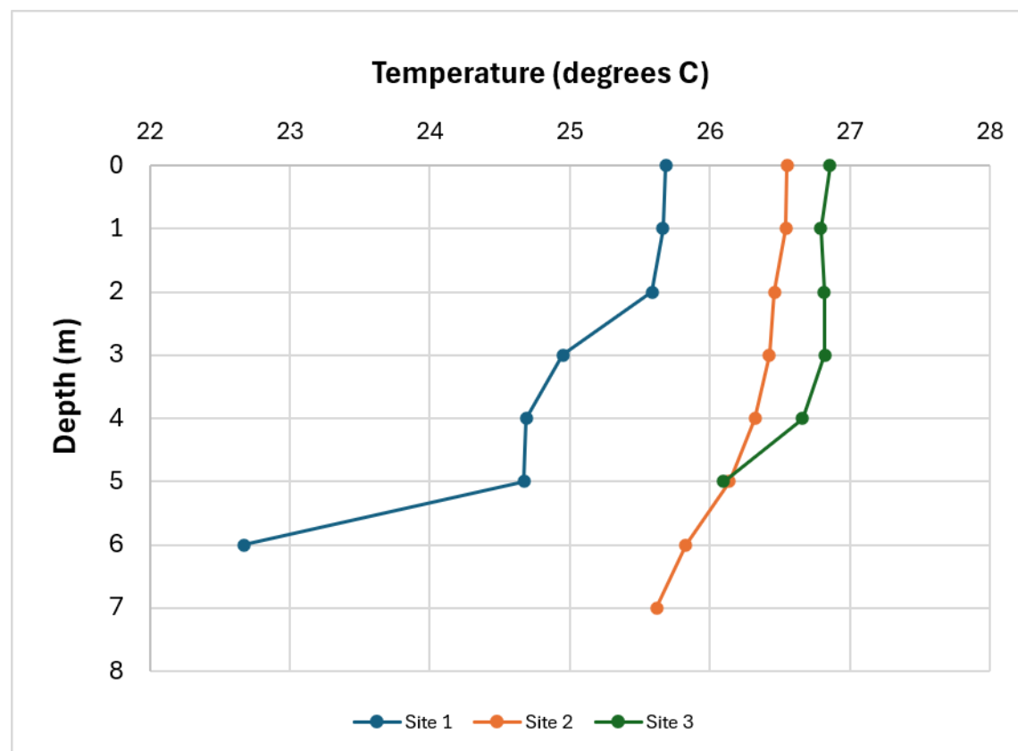
Figure 2. Graph of temperature measurements (reported in degrees Celsius) collected with depth on July 22, 2026. Pumphouse measurement reported in Table 2.
