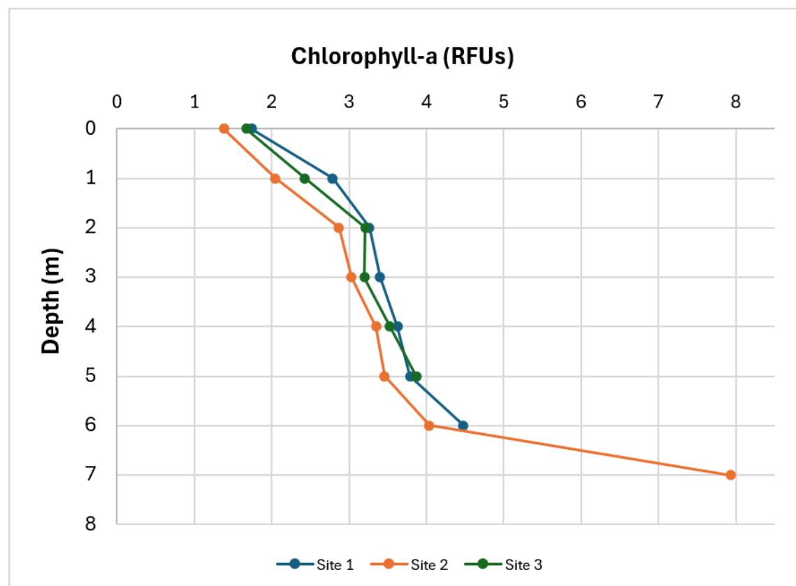
Figure 6. Graph of chlorophyll- a measurements (reported in relative fluorescence units; RFUs) collected with depth on July 22, 2026. Pumphouse measurement reported in Table 6.
