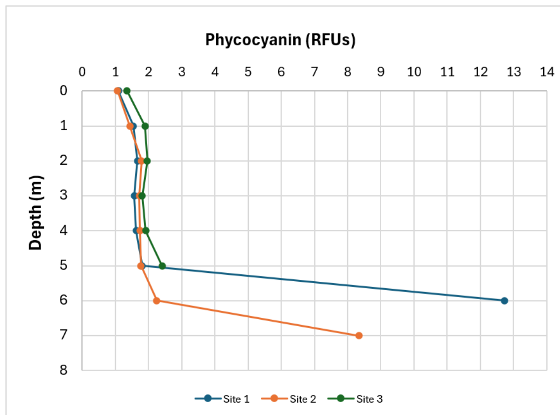
Figure 5. Graph of phycocyanin measurements (reported in relative fluorescence units; RFUs) collected with depth on July 22, 2026. Pumphouse measurement reported in Table 5.
