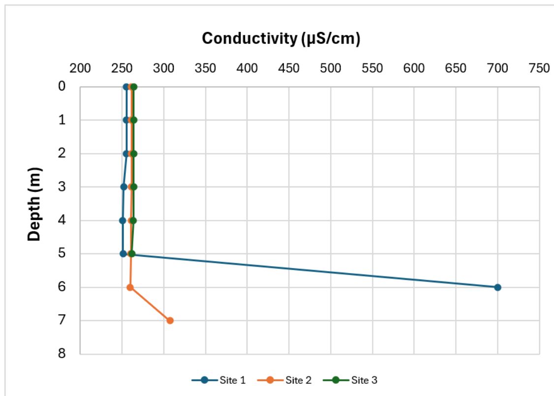
Figure 4. Graph of conductivity measurements (reported in \mu\text{S}/\text{cm} ) collected with depth on July 22, 2026. Pumphouse measurement reported in Table 4.
